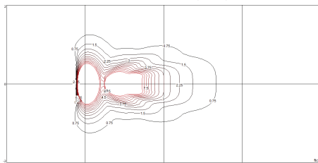
Dome Cutoff (DM)
