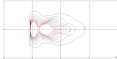
Round & Square Hood Cutoff (HDR & HDS)
