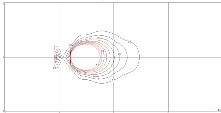
3/4 Cutoff w/o Integral Spread Lens (CNL2)
