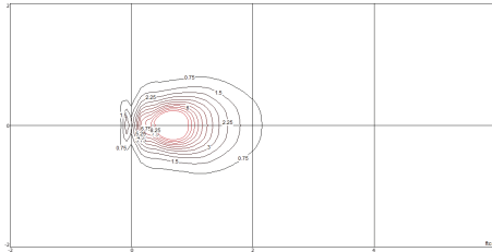
3/4 Cutoff w/ Integral Spread Lens (C2)
