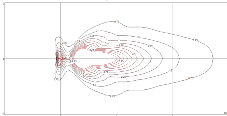
1/2 Cutoff w/o Integral Spread Lens (CNL1)
